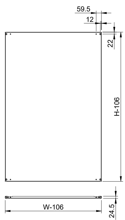
Mounting plate
