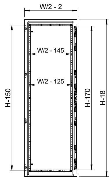
Inside right door view
