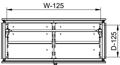
Sectional top view
