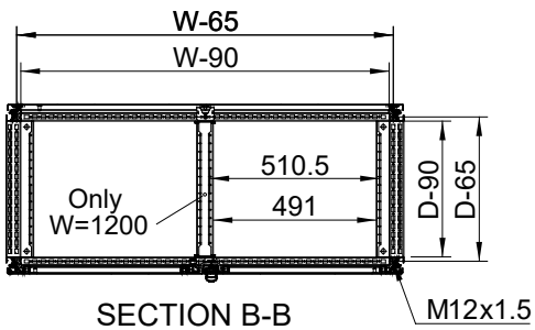
Sectional top view W=1600 (without bottom plates)
